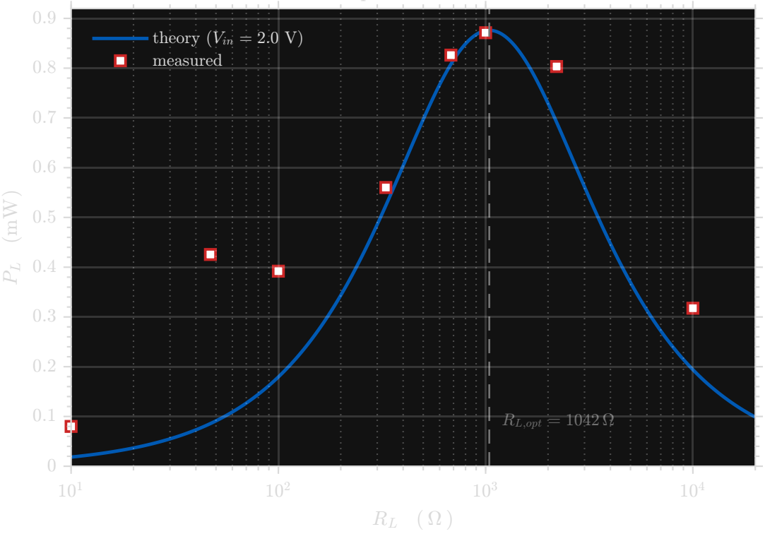
Case 1: load power vs. load resistance
